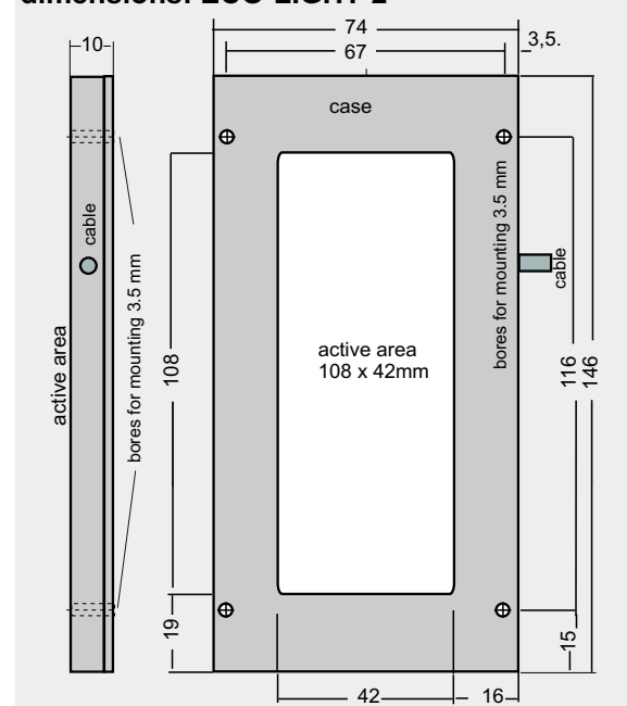
dimensions: ECO-LIGHT-2
